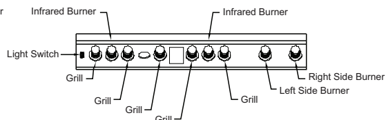
CR5000DS - 5 Burner Cart with Double Side Burners
