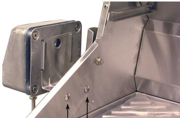
Attachment screws for rotis motor
